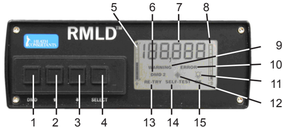
Figure 3-1 RMLD-IS front panel with display. (Note: the illustration shows all icons displayed simultaneously. During actual operation, only those symbols related to an active function will be displayed.)
