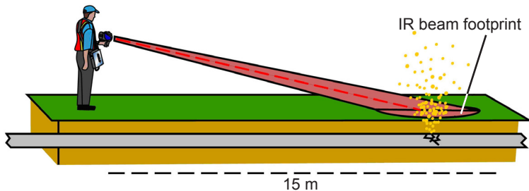
Figure 4-5: The ppm•m measurement value is the product of gas plume concentration multiplied by the distance that the beam passes through the gas (width of the gas plume) plus any background gas concentration level. The footprint of the laser beam increases with the scanning distance.
